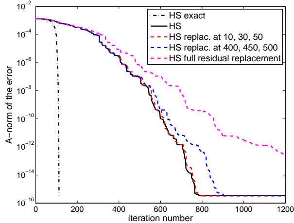
FIG. 3.5. The HS CG implementation and the modified CG implementations with residual replacement.
