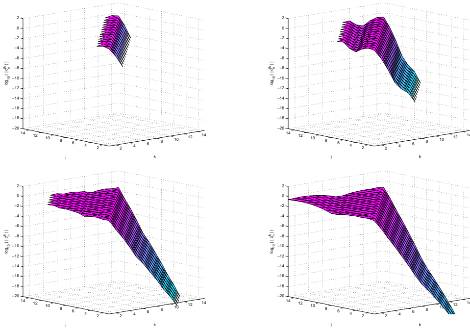
FIG. 3.2. The values \log_{10}(|c_n^{(jk)}|) for j, k = 1, \dots, N and n = 2 (top left), 6 (top right), 10 (bottom left), 14 (bottom right), computed when GMRES is applied to the 15 by 15 matrix T_1 = S + I + 0.01 S^T and r_0 = \text{rand}(15, 1) .
