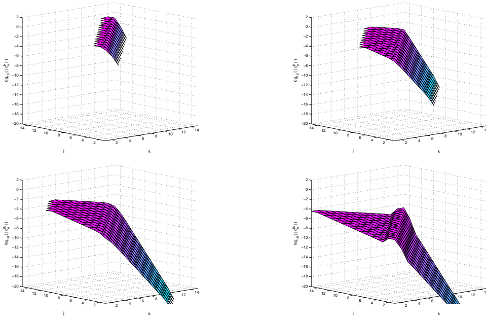
FIG. 3.3. The values \log_{10}(|c_n^{(jk)}|) for j, k = 1, \dots, N and n = 2 (top left), 6 (top right), 10 (bottom left), 14 (bottom right), computed when GMRES is applied to the 15 by 15 matrix T_2 = S + 2I + 0.01 S^T and r_0 = e .
