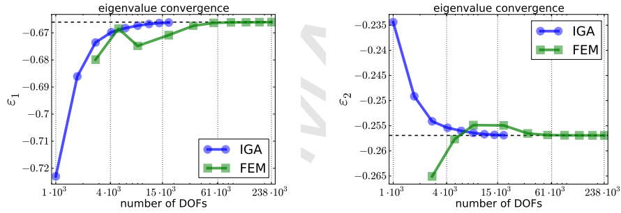
Figure 4: Convergence of eigenvalues \varepsilon_1 and \varepsilon_2 w.r.t. the number of DOFs.
