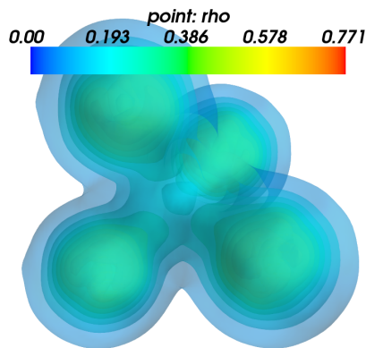
Figure 7: Tetrafluoromethane molecule: iso-surfaces of charge density \rho .
