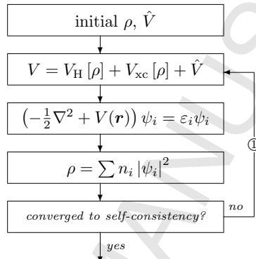
Figure 1: DFT, iterative self-consistent scheme.
