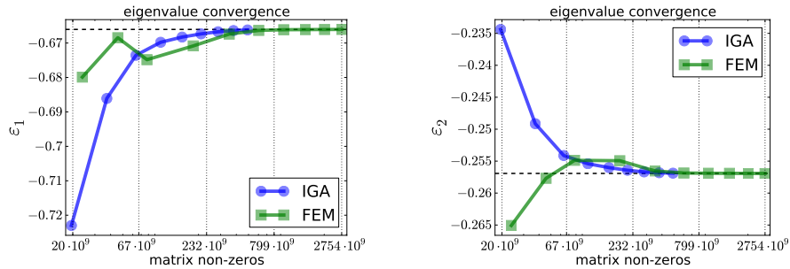
Figure 5: Convergence of eigenvalues \varepsilon_1 and \varepsilon_2 w.r.t. the number of non-zeros of the matrices.
