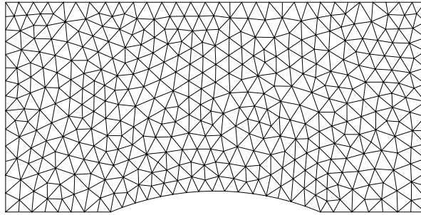
FIG. 5.8. Coarse triangular mesh (784 triangles) in the GAMM channel
