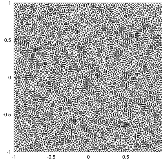
FIG. 5.3. Triangulation used for the numerical solution
