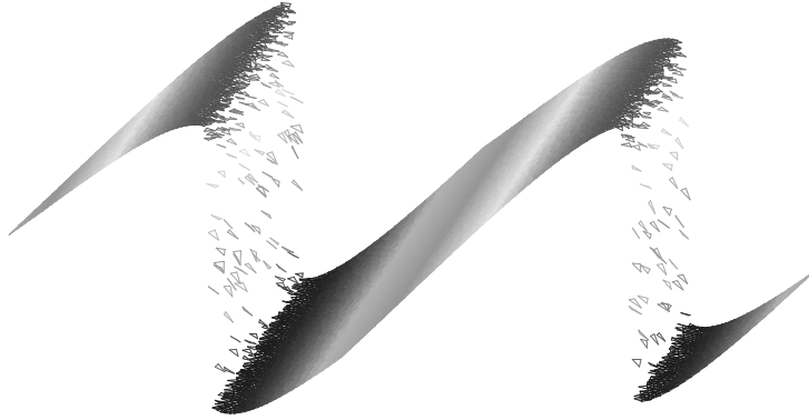
FIG. 5.5. Numerical solution of the problem from Example 5.4 computed by DGFEM with limiting, plotted at t = 0.45
