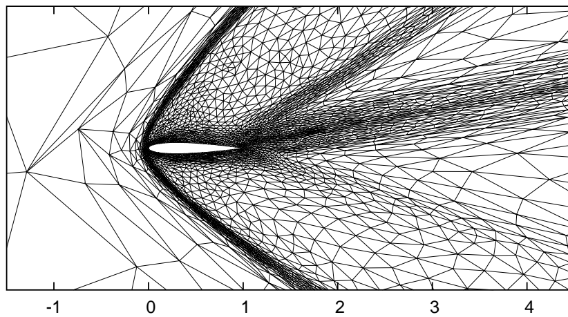
FIG. 5.13. Viscous supersonic flow past the profile NACA 0012: triangulation
