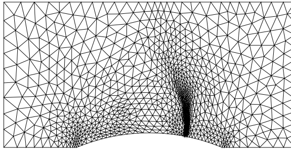
FIG. 5.11. Adapted triangular mesh (2131 triangles) in the GAMM channel mesh adaptation (AMA) technique. Fig. 5.14 shows the Mach number isolines. Here we see a shock wave in front of the profile, wake and a shock wave leaving the profile.
