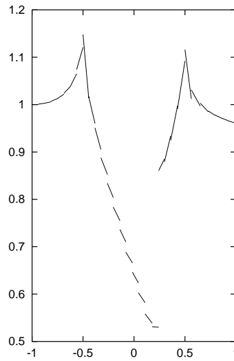
FIG. 5.10. Density distribution along the lower wall in the GAMM channel with the use of a bilinear mapping at \partial\Omega
