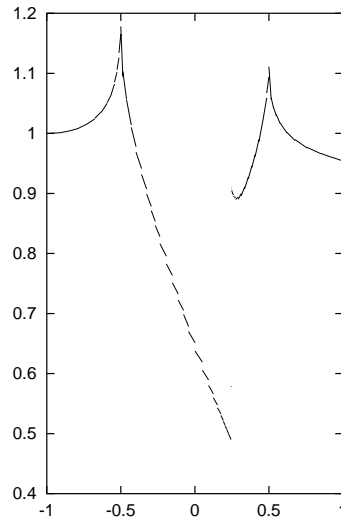
FIG. 5.12. Density distribution along the lower wall in the GAMM channel with the use of a bilinear mapping on an adapted mesh
