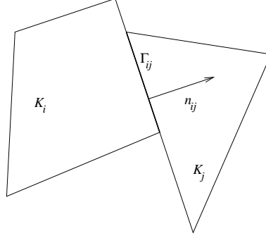
FIG. 5.1. Neighbouring elements K_i, K_j
