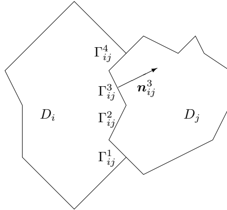
FIG. 4.1. Neighbouring finite volumes in 2D, \Gamma_{ij} = \bigcup_{\alpha=1}^4 \Gamma_{ij}^\alpha
