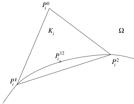
FIG. 5.6. Triangle K_i lying on a curved part of \partial\Omega
