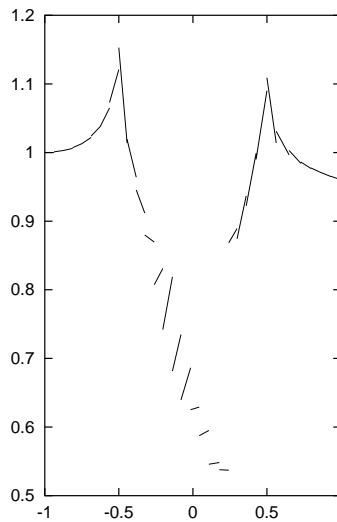
FIG. 5.9. Density distribution along the lower wall in the GAMM channel without the use of a bilinear mapping at \partial\Omega
