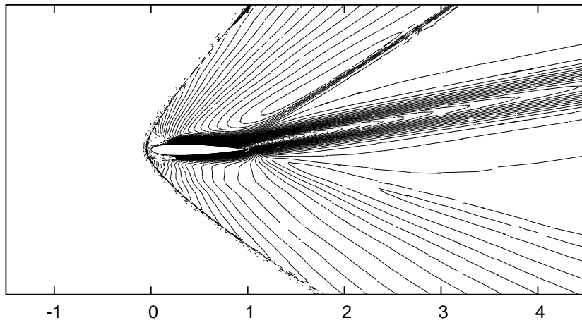
FIG. 5.14. Viscous supersonic flow past the profile NACA 0012: Mach number isolines
