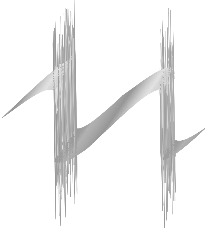
FIG. 5.4. Numerical solution of the problem from Example 5.4 computed by DGFEM, plotted at t = 0.45
